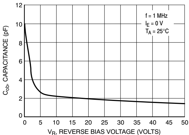
Figure 29. Output Capacitance
